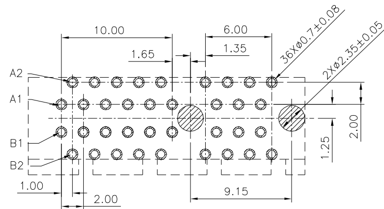
Recommended P.C.B. Layout(Component Side) (PCB Board Tolerance±0.05)
