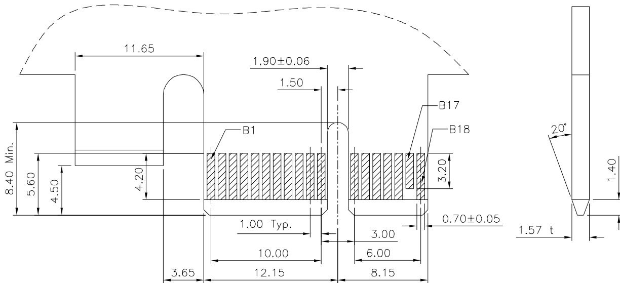
Recommended Edge Card Pattern(Primary Side)
