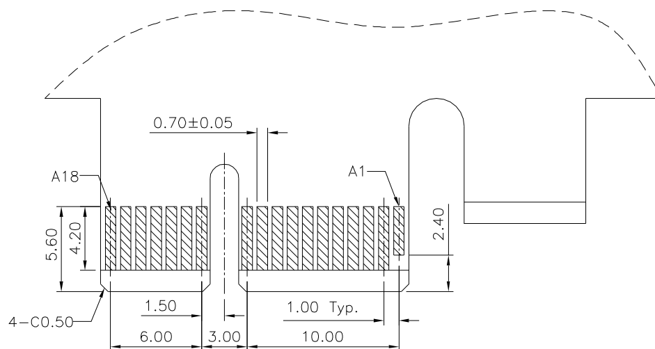
Recommended Edge Card Pattern(Secondary Side)
