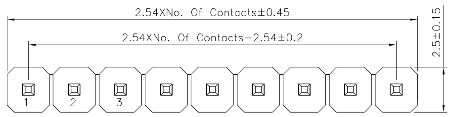
Recommended P.C.B. Layout(Top View) (PCB Board Tolerance±0.05)
