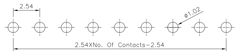
Recommended P.C.B. Layout(Top View) (PCB Board Tolerance±0.05)
