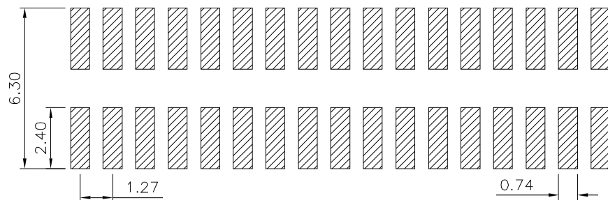
Recommended P.C.B. Layout(Top Side) (PCB Board Tolerance±0.05)
