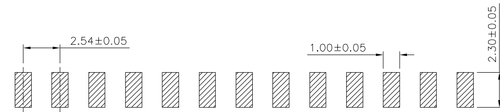
Recommended P.C.B. Layout (PCB Board Tolerance±0.05)
