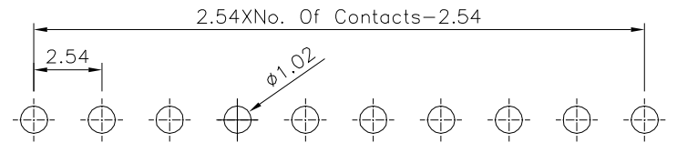
△ Recommended P.C.B. Layout (Top View) (PCB Board Tolerance ±0.05)
