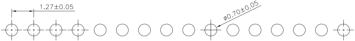
Recommended P.C.B. Layout
