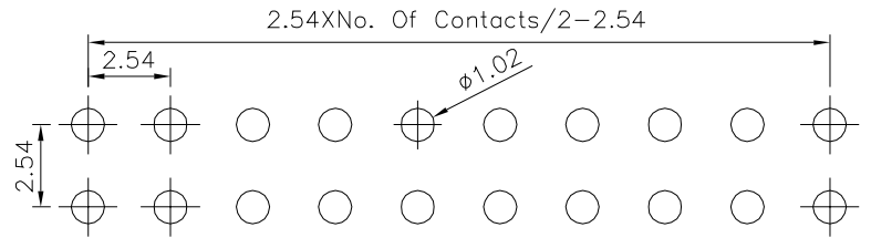
Recommended P.C.B. Layout (Top View) (PCB Board Tolerance ±0.05) ⚠
