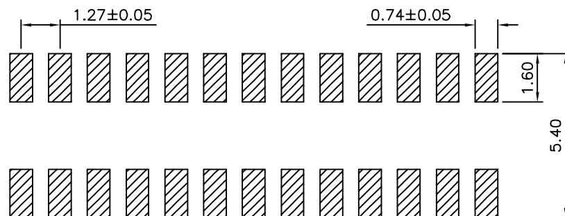
Recommended P.C.B. Layout (PCB Board Tolerance±0.05)⚠
