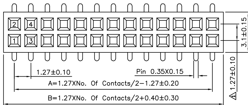
Recommended P.C.B. Layout (PCB Board Tolerance±0.05)⚠
