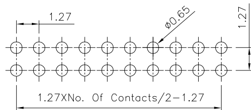
Recommended P.C.B. Layout(Top View) (PCB Board Tolerance±0.05)
