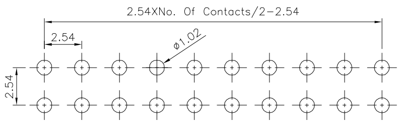
⚠ Recommended P.C.B. Layout(Top View) (PCB Board Tolerance±0.05)
