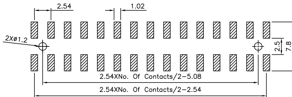
Recommended P.C.B. Layout(Top View) (PCB Board Tolerance±0.05)
