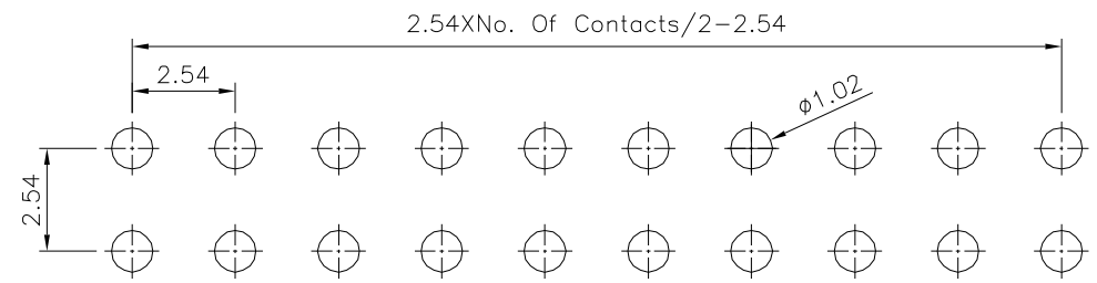
Recommended P.C.B. Layout(Top View) (PCB Board Tolerance±0.05)
