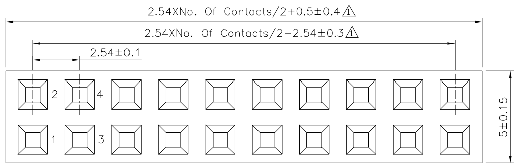
Recommended P.C.B. Layout(Top View) (PCB Board Tolerance±0.05)
