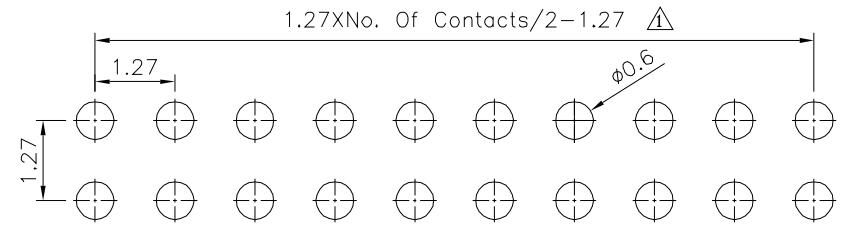
Recommended P.C.B. Layout(Top View) (PCB Board Tolerance±0.05)
