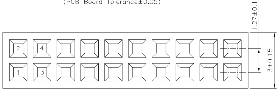
Recommended P.C.B. Layout(Top View) (PCB Board Tolerance±0.05)
