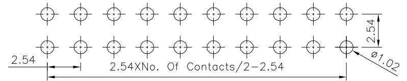
Recommended P.C.B. Layout(Top View) (PCB Board Tolerance±0.05)
