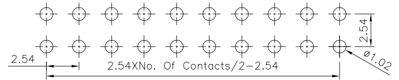
Recommended P.C.B. Layout (Top View) (PCB Board Tolerance ±0.05)
