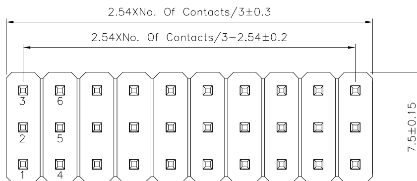
Recommended P.C.B. Layout(Top View) (PCB Board Tolerance±0.05)
