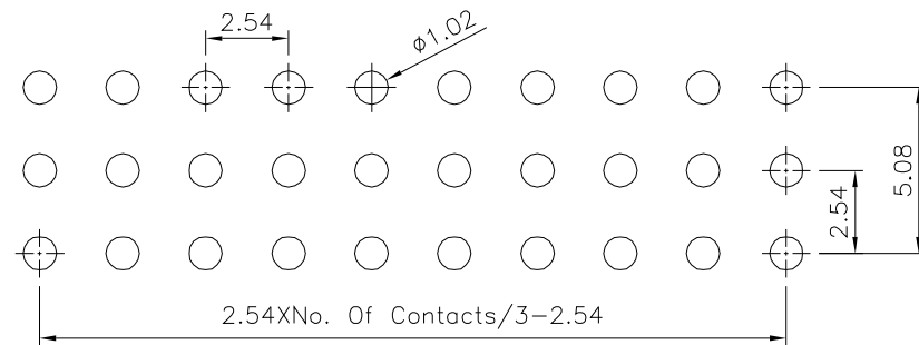
Recommended P.C.B. Layout(Top View) (PCB Board Tolerance±0.05)
