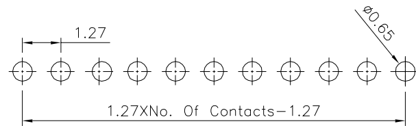
Recommended P.C.B. Layout(Top View) (PCB Board Tolerance±0.05)
