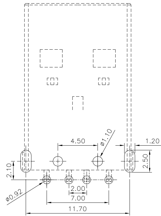
Recommended P.C.B. Layout Tolerances: ±0.10
