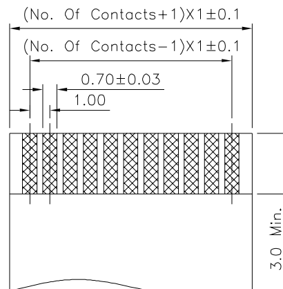
Applicable FPC/FFC Thickness:0.25~0.35mm
