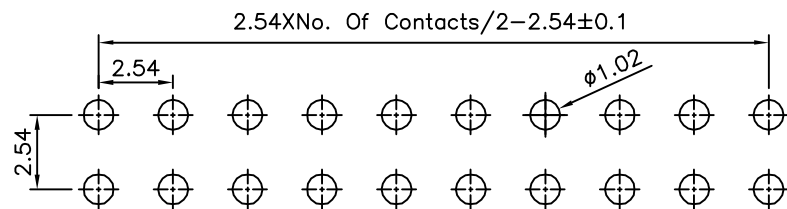
Recommended P.C.B. Layout(Top View) (PCB Board Tolerance±0.05)
