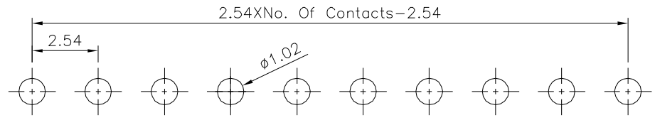
⚠️ Recommended P.C.B. Layout (Top View) (PCB Board Tolerance ±0.05)
