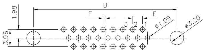
Recommended P.C.B. Layout(26,44,62 Pin)
