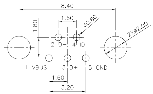
Recommended P.C.B. Layout (Thickness=1.00mm)
