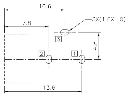
Recommended P.C.B. Layout (Bottom View) Unspecified Tolerance:±0.05
