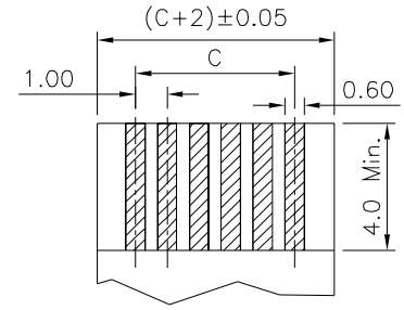
FPC/FFC T=0.30±0.05
