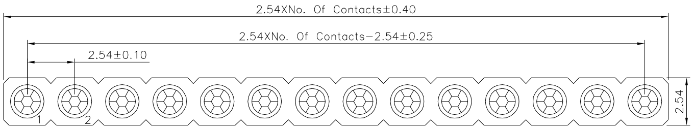
Recommended P.C.B. Layout △ Tolerance ±0.05
