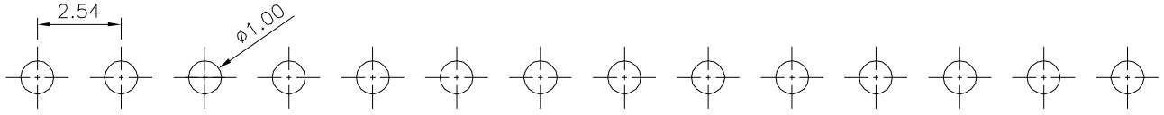
Recommended P.C.B. Layout △ Tolerance ±0.05
