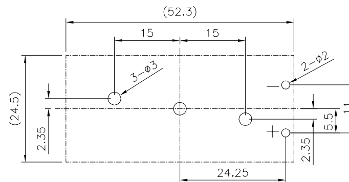
Recommended P.C.B. Layout(Top Side)
