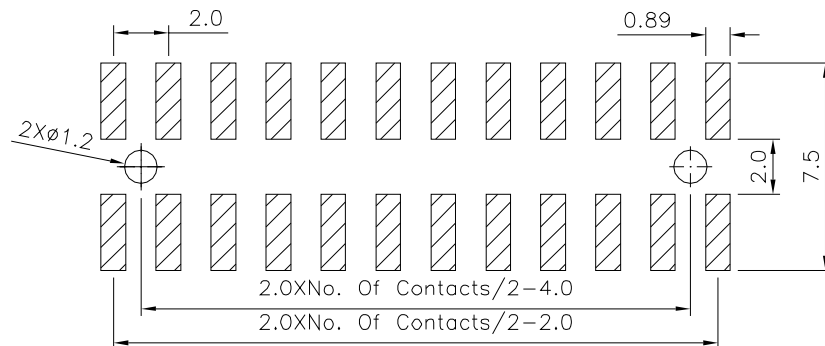
Recommended P.C.B Layout(Top View) (PCB Board Tolerance±0.05)
