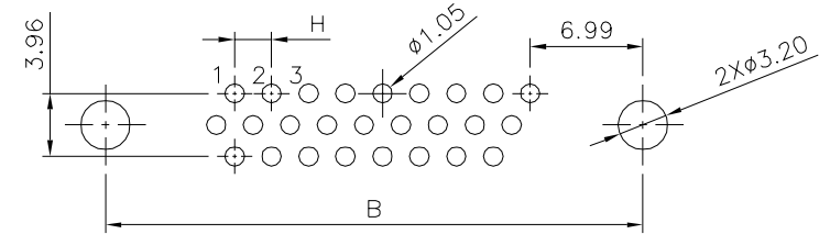
Recommended P.C.B. Layout 26 Pin
