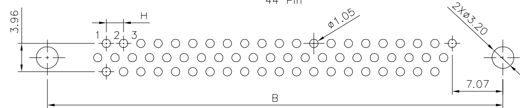
Recommended P.C.B. Layout 62 Pin
