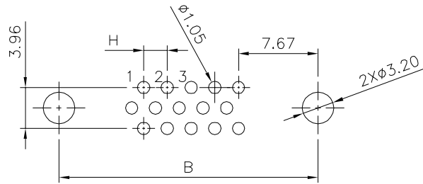
Recommended P.C.B. Layout 15 Pin
