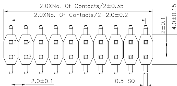
Recommended P.C.B. Layout(Top View) (PCB Board Tolerance±0.05)
