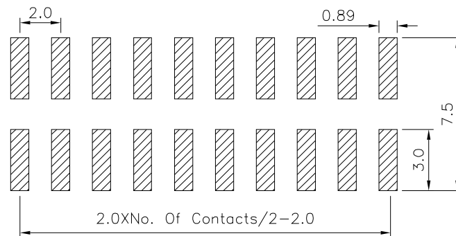
Recommended P.C.B. Layout(Top View) (PCB Board Tolerance±0.05)
