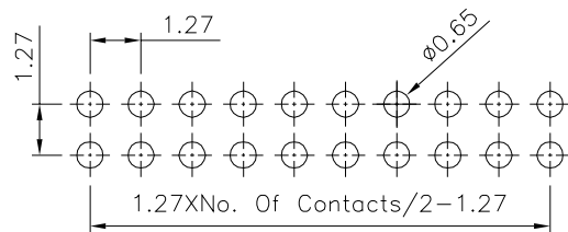
Recommended P.C.B. Layout(Top View) (PCB Board Tolerance±0.05)
