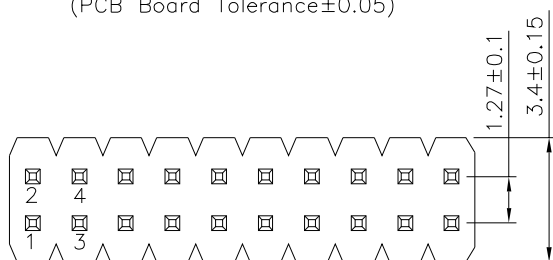
Recommended P.C.B. Layout(Top View) (PCB Board Tolerance±0.05)
