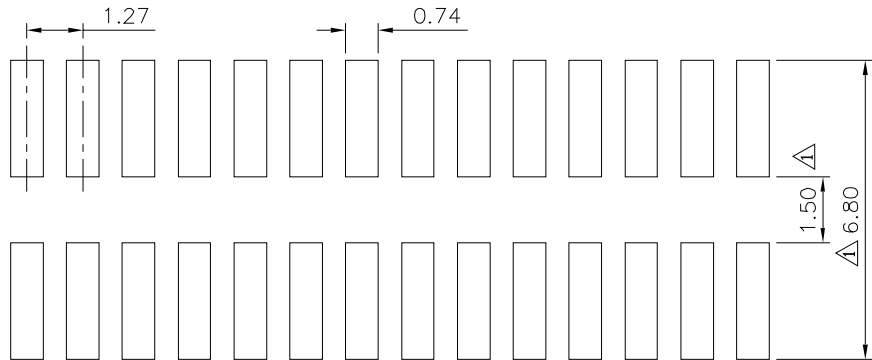
Recommended P.C.B. Layout (PCB Board Tolerance±0.05)
