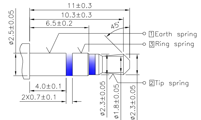
Matching Plug
