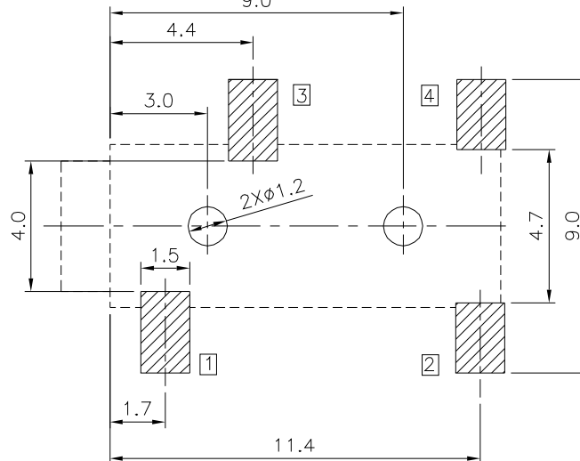
Recommended P.C.B. Layout(Top Side) (PCB Board Tolerance±0.05)
