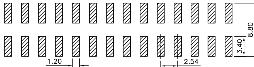
Recommended P.C.B. Layout(Top Side) (PCB Board Tolerance±0.05)
