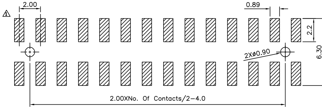
Recommended P.C.B. Layout(Top Side) (PCB Board Tolerance ±0.05)
