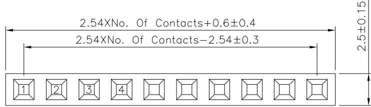
Recommended P.C.B. Layout(Top View) (PCB Board Tolerance±0.05)
