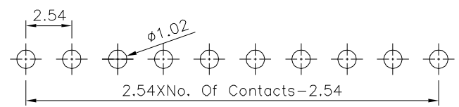
Recommended P.C.B. Layout(Top View) (PCB Board Tolerance±0.05)
