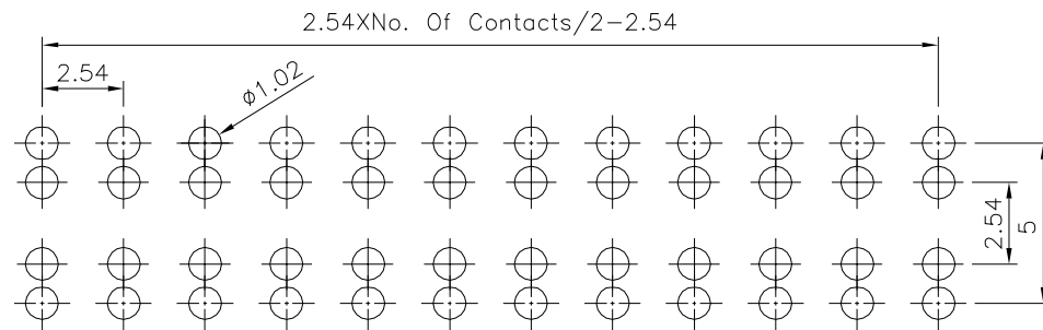
Recommended P.C.B. Layout(Top View) (PCB Board Tolerance \pm 0.05 )
