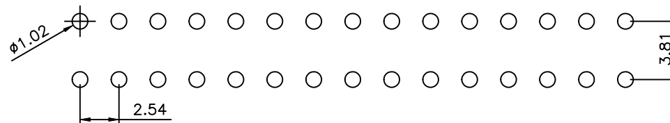
Recommended P.C.B Layout(Top Side) (PCB Board Tolerance±0.05)
