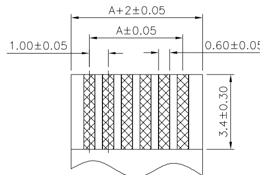
△ FPC/FFC T=0.30±0.05
