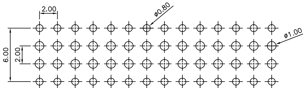
Recommended P.C.B. Layout(Top Side) \Delta (PCB Board Tolerance \pm 0.05 )
