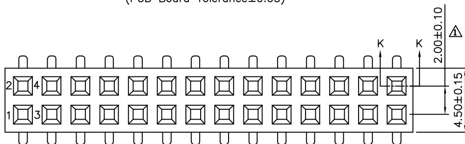
Recommended P.C.B. Layout(Top Side) \Delta (PCB Board Tolerance \pm 0.05 )
