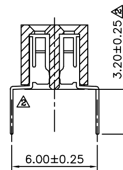
Section L-L
