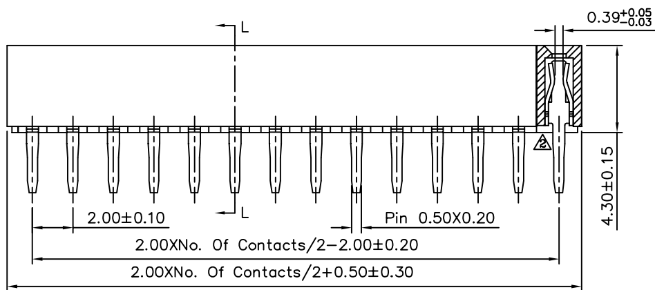
Section K-K
