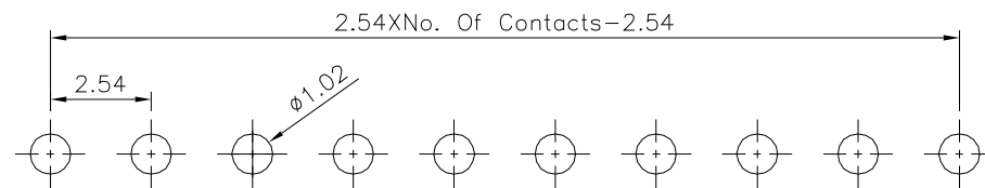
Recommended P.C.B. Layout(Top View) (PCB Board Tolerance±0.05)
