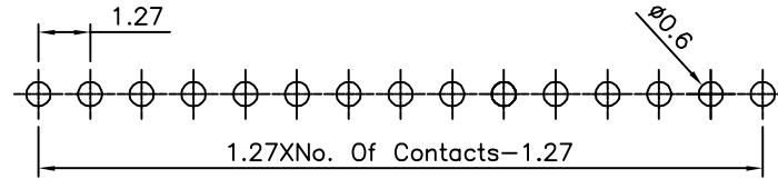
Recommended P.C.B. Layout(Top View) (PCB Board Tolerance±0.05)
