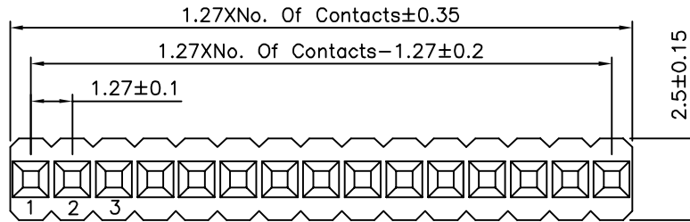
Recommended P.C.B. Layout(Top View) (PCB Board Tolerance±0.05)
