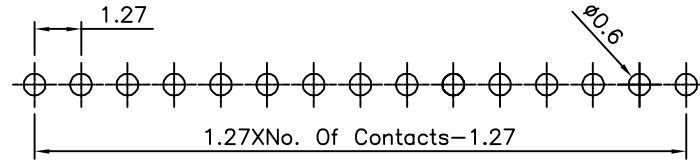
Recommended P.C.B. Layout(Top View) (PCB Board Tolerance±0.05)
