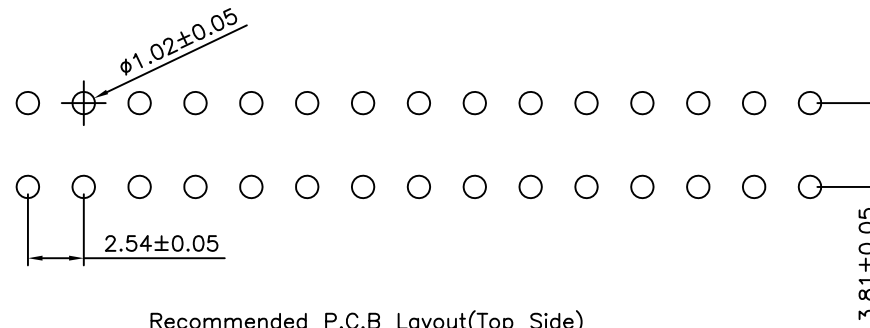
Recommended P.C.B Layout(Top Side)
