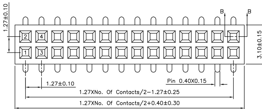
△ Recommended P.C.B Layout(Top Side) (PCB Board Tolerance:±0.05)
