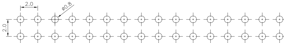
Recommended P.C.B. Layout
