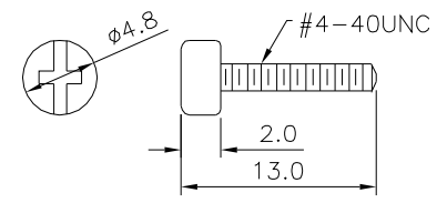
△ Screw: For O.D. 7.0/9.0/10.0mm
