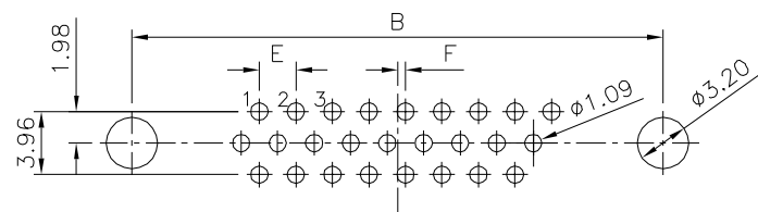
△△ Recommended P.C.B. Layout(26,44,62 Pin)
