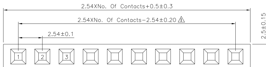
Recommended P.C.B. Layout(Top View) (PCB Board Tolerance±0.05)
